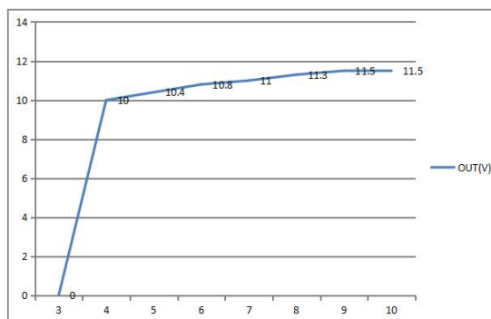
Output voltage curve
