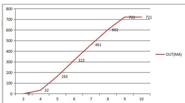
Output current curve
